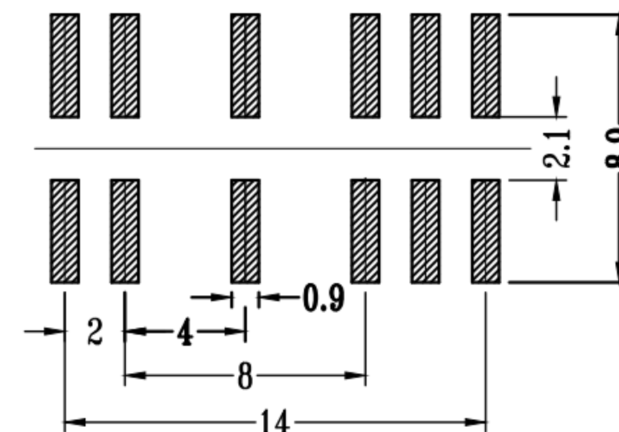
P.C.B LAYOUT BOTTOM VIEW
